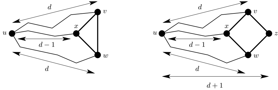
FIGURE 1. Triangle and quadrangle conditions
