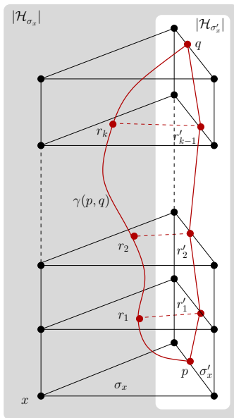
FIGURE 6. To the proof of Claim 2
