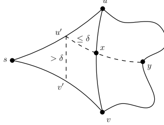
Fig. 3. To the proof of Proposition 3
