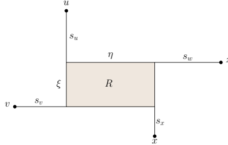
Fig. 1. Realization of a 4-point metric in the rectilinear plane.
