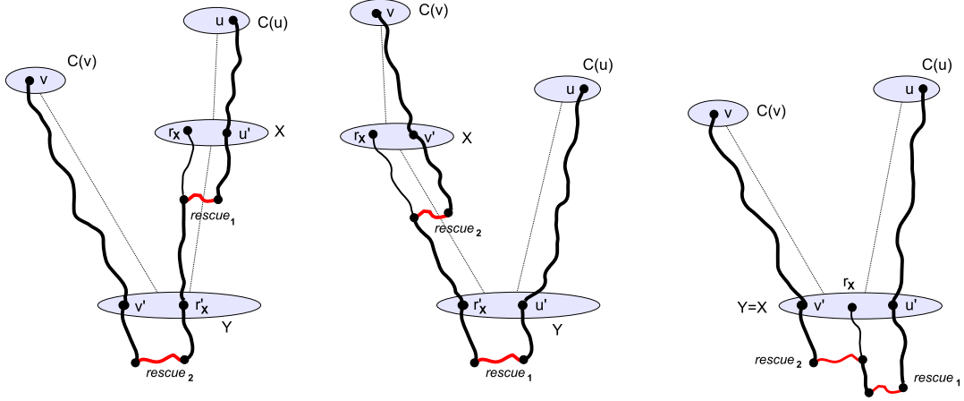
Fig. 5. The three possible locations of cluster X on the path of \Gamma between C(u) and C(v) (with respect to Y ). The routing path induced by the scheme is indicated in all three cases. The paths rescue_1 and rescue_2 are shown in red. The black parts are paths from the spanning tree \mathcal{VT} of G . Note that, we show rooted trees growing upward, so the roots are on bottom.
