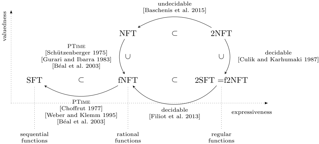
Fig. 3. A landscape of transducers of finite words.
