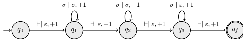
Fig. 2. A two-way transducer T_2 for f_{mir} .
