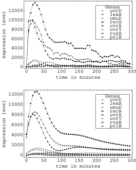
Fig. 4. Top: mean expression profiles of the 8 genes corresponding to the second second data set. Bottom: learned profiles from this data set for \lambda = 100 . The vertical scale has no absolute meaning, since we took the (dGFP/dt)/OD values of Ronen et al. (2002), which are proportional to the expression levels of the genes as explained previously.
