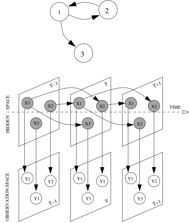
Fig. 2. A 3 genes network, represented as a static Bayesian network (top), and as a dynamic Bayesian network (bottom).
