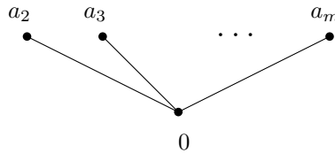
FIGURE 1. The poset \text{Ap}(\mathcal{S}, m) .
