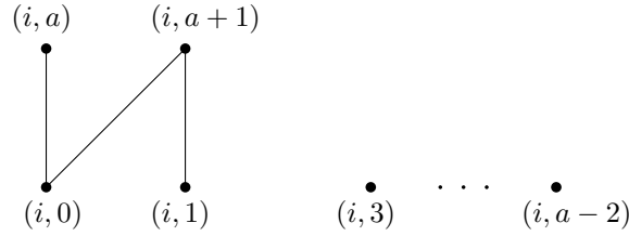
FIGURE 9. P \cap \mathcal{S}_i in case (2).
