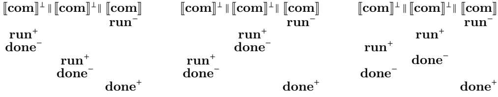
■ Figure 2 Some plays in [[\parallel]]_{\mathbf{GM}}
