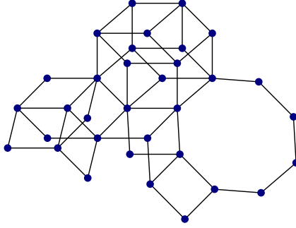
FIGURE 1. The tope graph M of a CUOM
