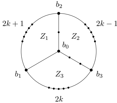
Figure 3: The Heldrlín-Pultr graph H^k .
