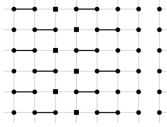
Figure 10: Sets of edges of T_{8,6} for Lemma 20, with vertices in V' represented as squares.
