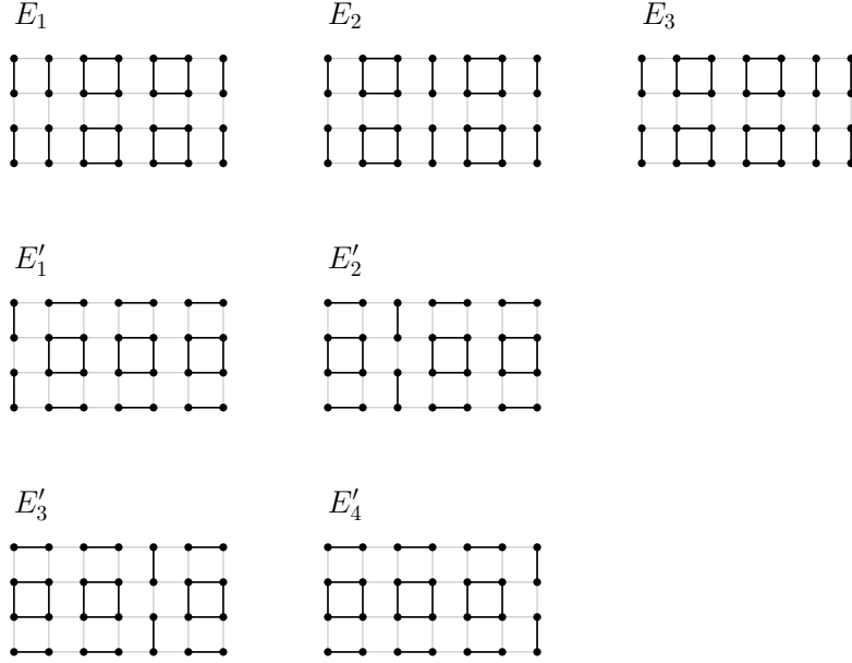
Figure 3: Spanning subgraphs of G_{7,4} for Lemma 10.
