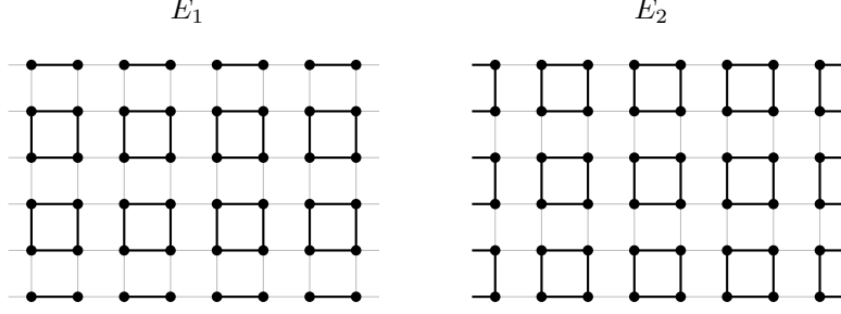
Figure 6: Spanning subgraphs of Y_{8,6} for Lemma 15.
