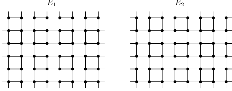
Figure 9: Spanning subgraphs of T_{8,6} for Lemma 19.
