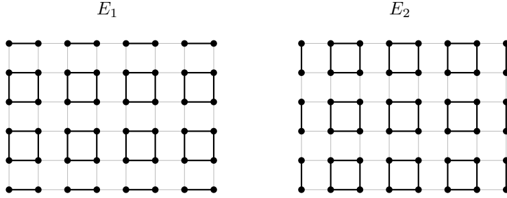
Figure 2: Spanning subgraphs of G_{8,6} for Lemma 9.
