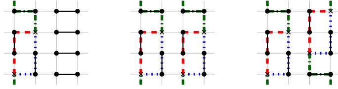
Figure 12: Toroidal grid T_{4,4} with the three possible sets of unsaturated vertices, corresponding maximal matchings, and augmenting path forests, for Lemma 22.
