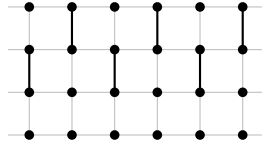
Figure 7: Matching M in Y_{6,4} for Lemma 16.
