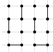
Figure 11: Edge set E_1 for Lemma 21.
