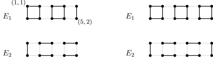
Figure 1: Spanning subgraphs of G_{5,2} and G_{6,2} for Lemma 8.
