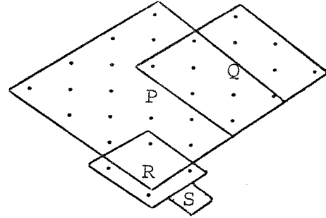
Fig. 2. A region defined by maximal neighborhoods of the points P, Q, R, S , with radii 3, 2, 1, and 0.
