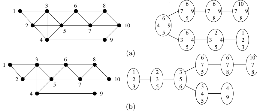
Fig. 1. (a) A graph of tree-width 3 and the corresponding tree-decomposition. (b) A 2-PST of the graph given in (a), and one tree-decomposition.
