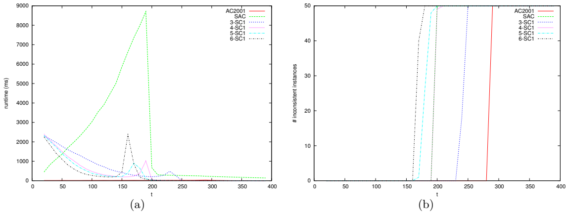
Fig. 3. Results obtained for random instances of classes (200,20,5970,t) : (a) runtime in ms and (b) number of detected inconsistent instances.
