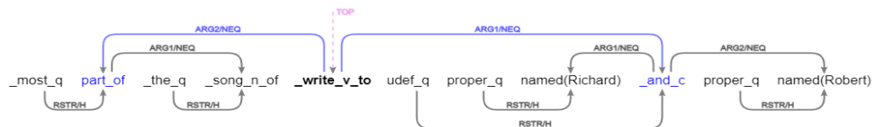
e. DMRS of sentence 5. “Most of the songs were written by Richard M. Sherman and Robert B. Sherman”.
