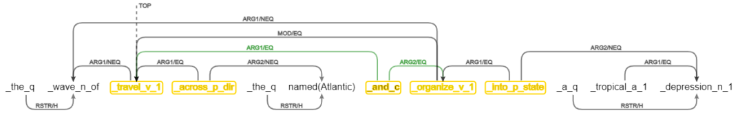
a. DMRS of sentence 1. “The wave traveled across the Atlantic, and organized into a tropical depression off the northern coast of Haiti on September 13”.
