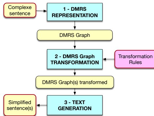
Figure 1. Steps of the syntactic simplification method.
