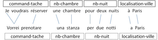
Figure 1: Example of concepts projection from source to target language.
